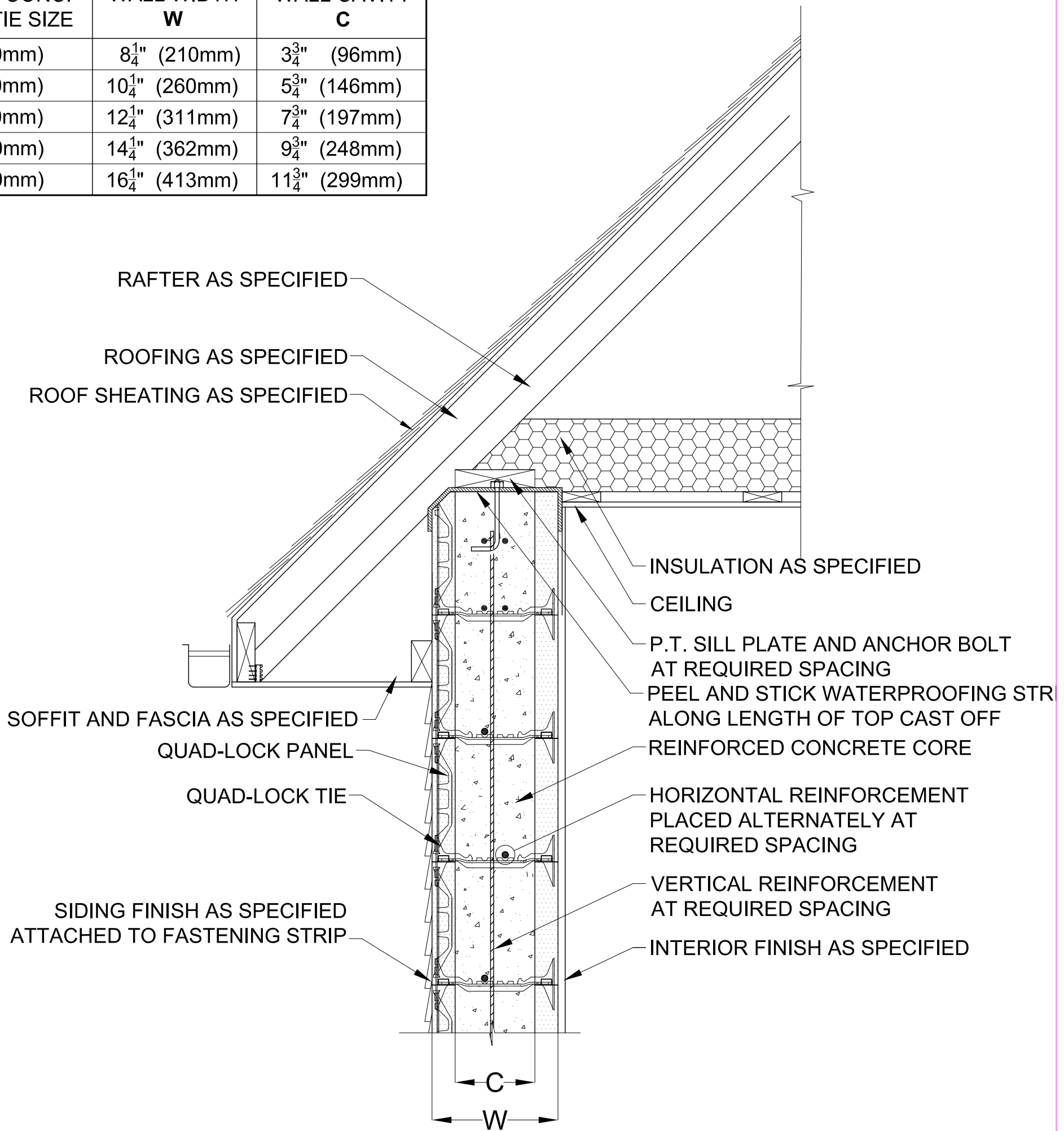
1 SECTION DETAIL 6.1.1
