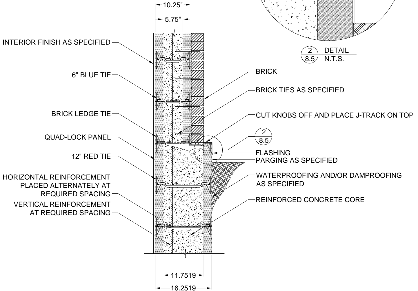
1 8.5 SECTION DETAIL 3/4" = 1'
