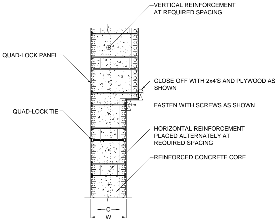
1 CONNECTION DETAIL 9.3 3/4" = 1'
