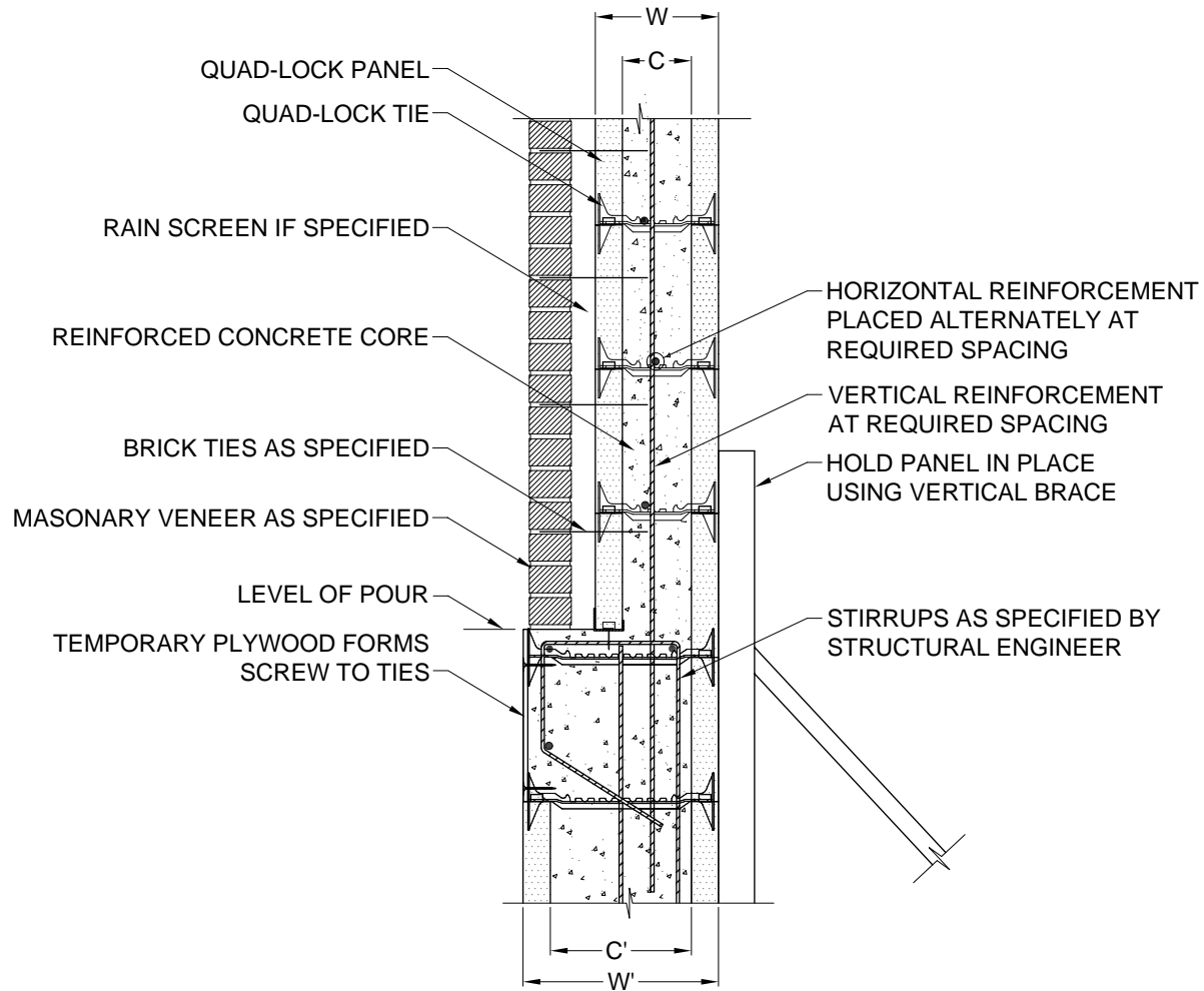
1 8.1 SECTION DETAIL 3/4" = 1'
