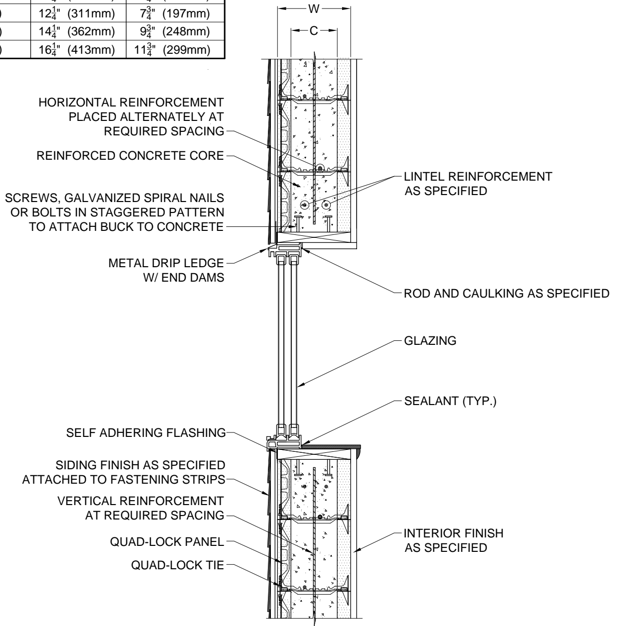
1 SECTION DETAIL 7.3 3/4" = 1'
