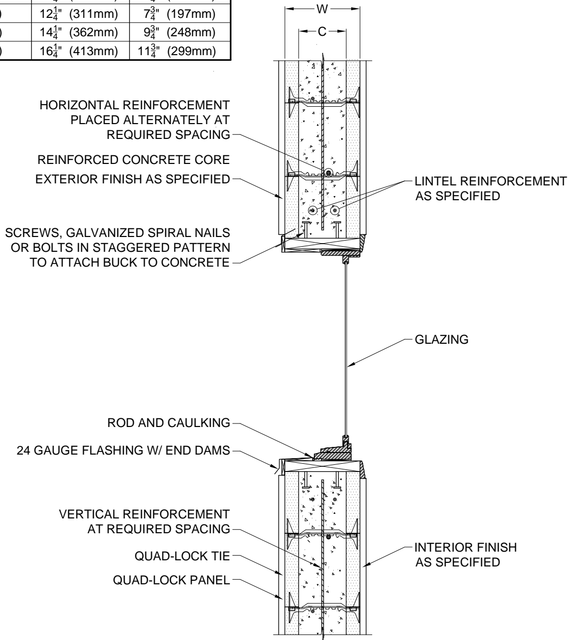
1 SECTION DETAIL 7.2 3/4" = 1'
