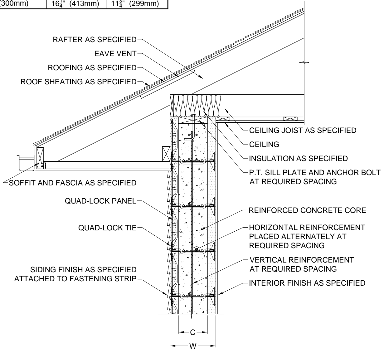
1 SECTION DETAIL 6.1 3/4" = 1'
