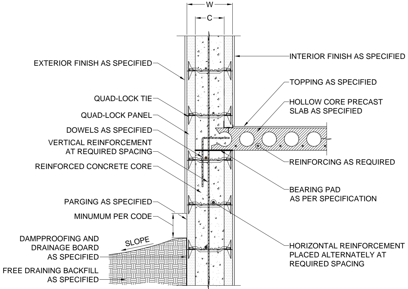
1 5.4 CONNECTION DETAIL 3/4" = 1'
