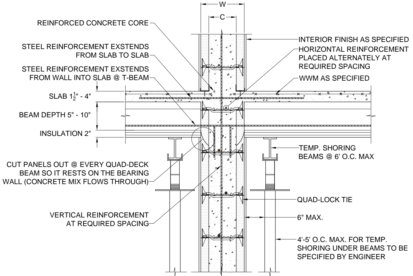
1 CONNECTION DETAIL 4.3 3/4" = 1'
