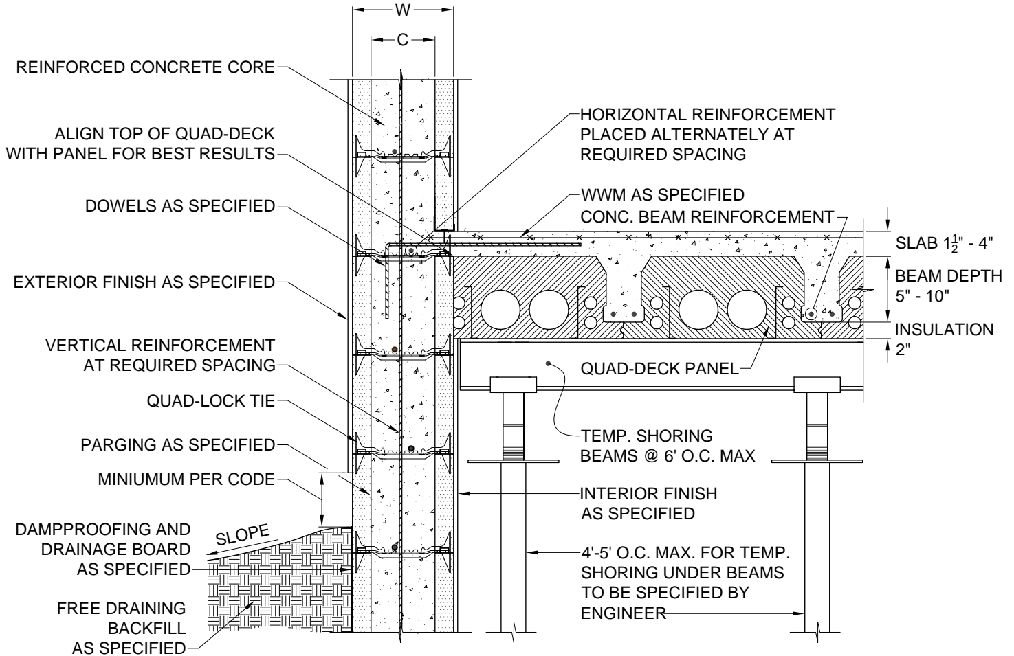
1 CONNECTION DETAIL 4.2 3/4" = 1'
