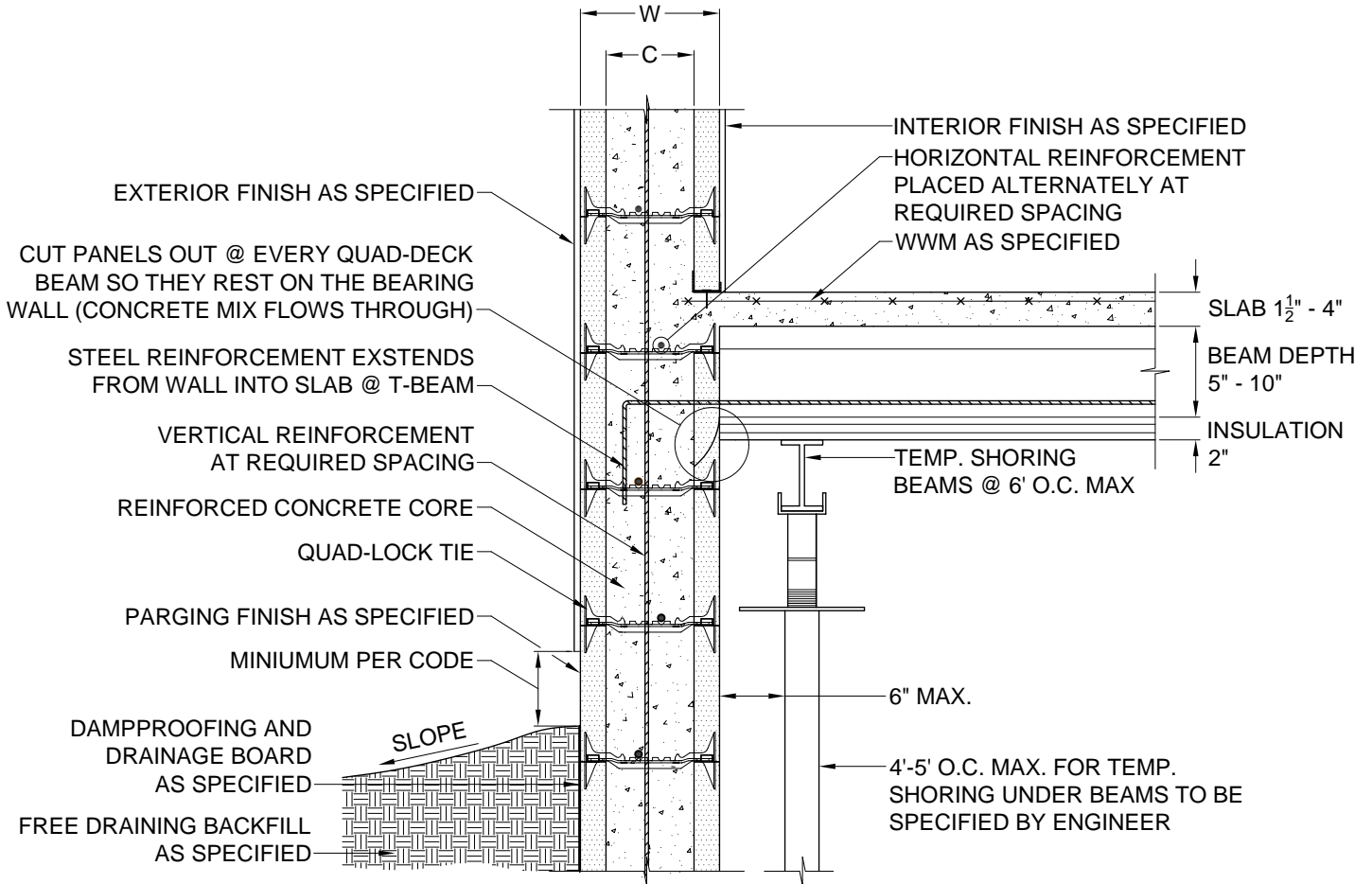
1 CONNECTION DETAIL 4.1 3/4" = 1'
