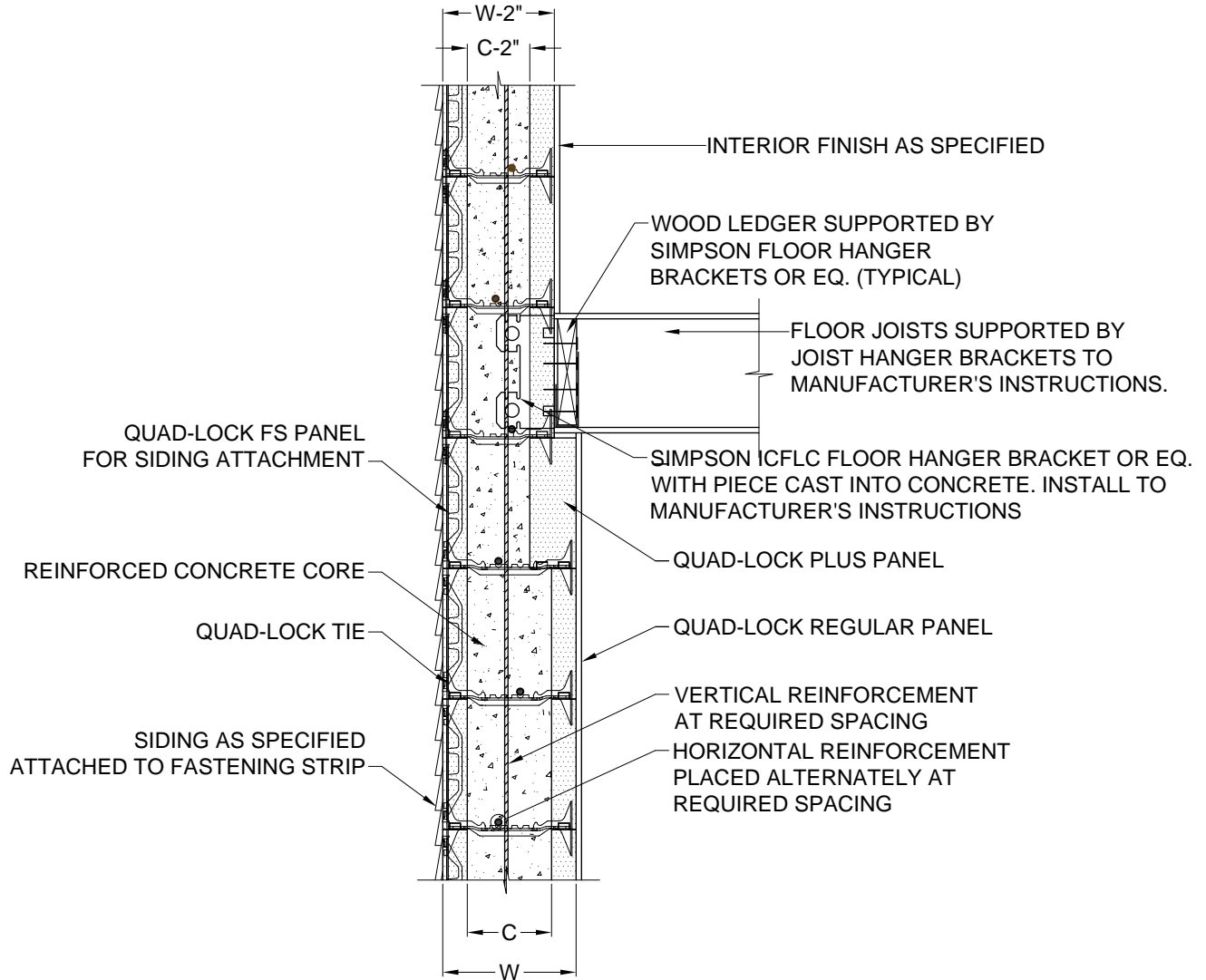
1 SECTION DETAIL 3.5 3/4" = 1'
