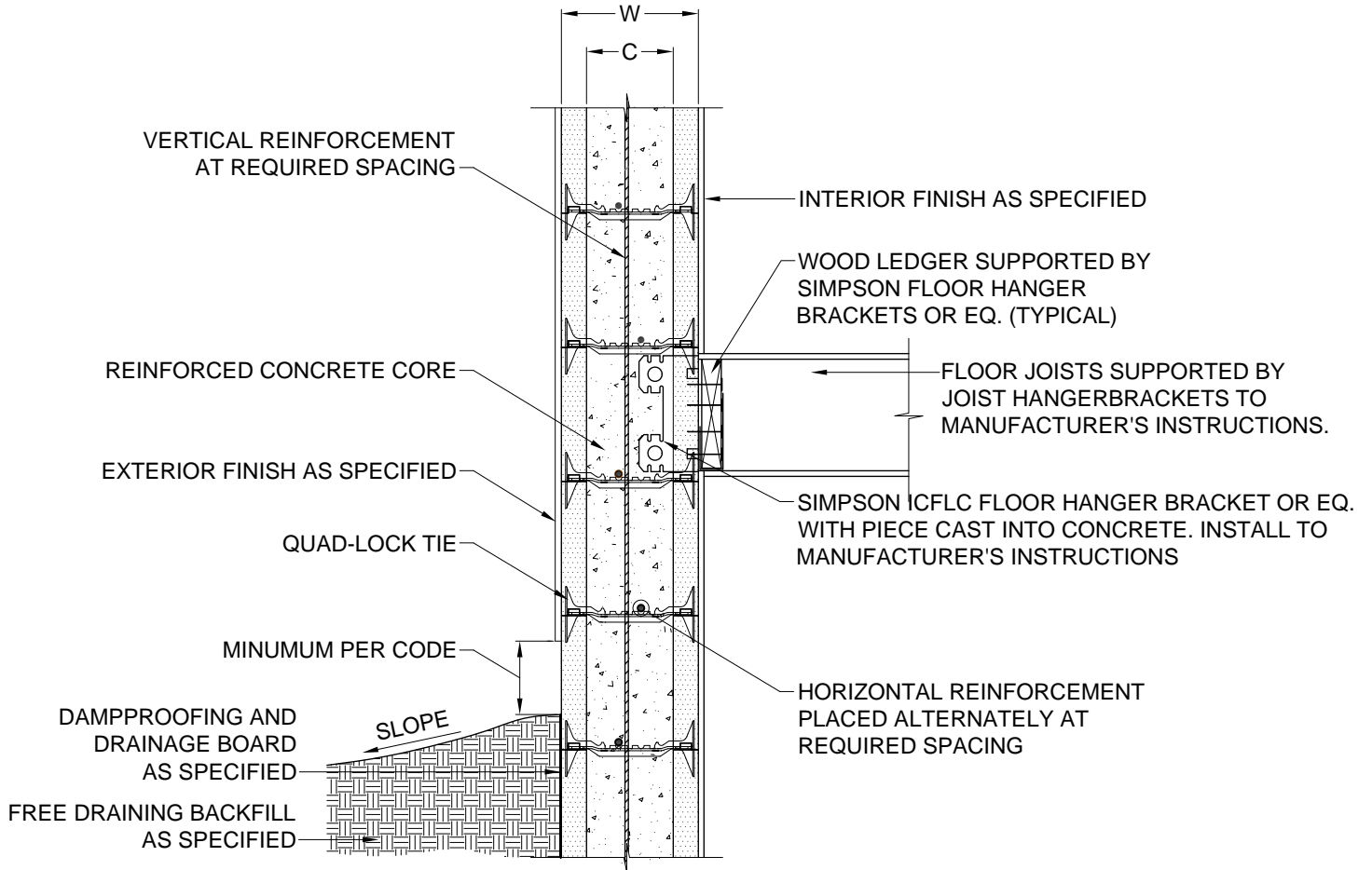
1 CONNECTION DETAIL 3.4 3/4" = 1'
