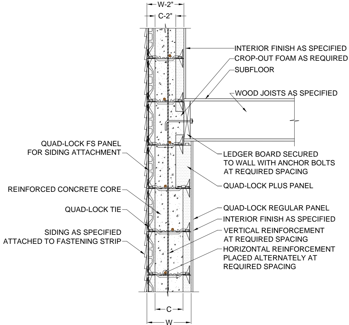
1 SECTION DETAIL 3.3 3/4" = 1'
