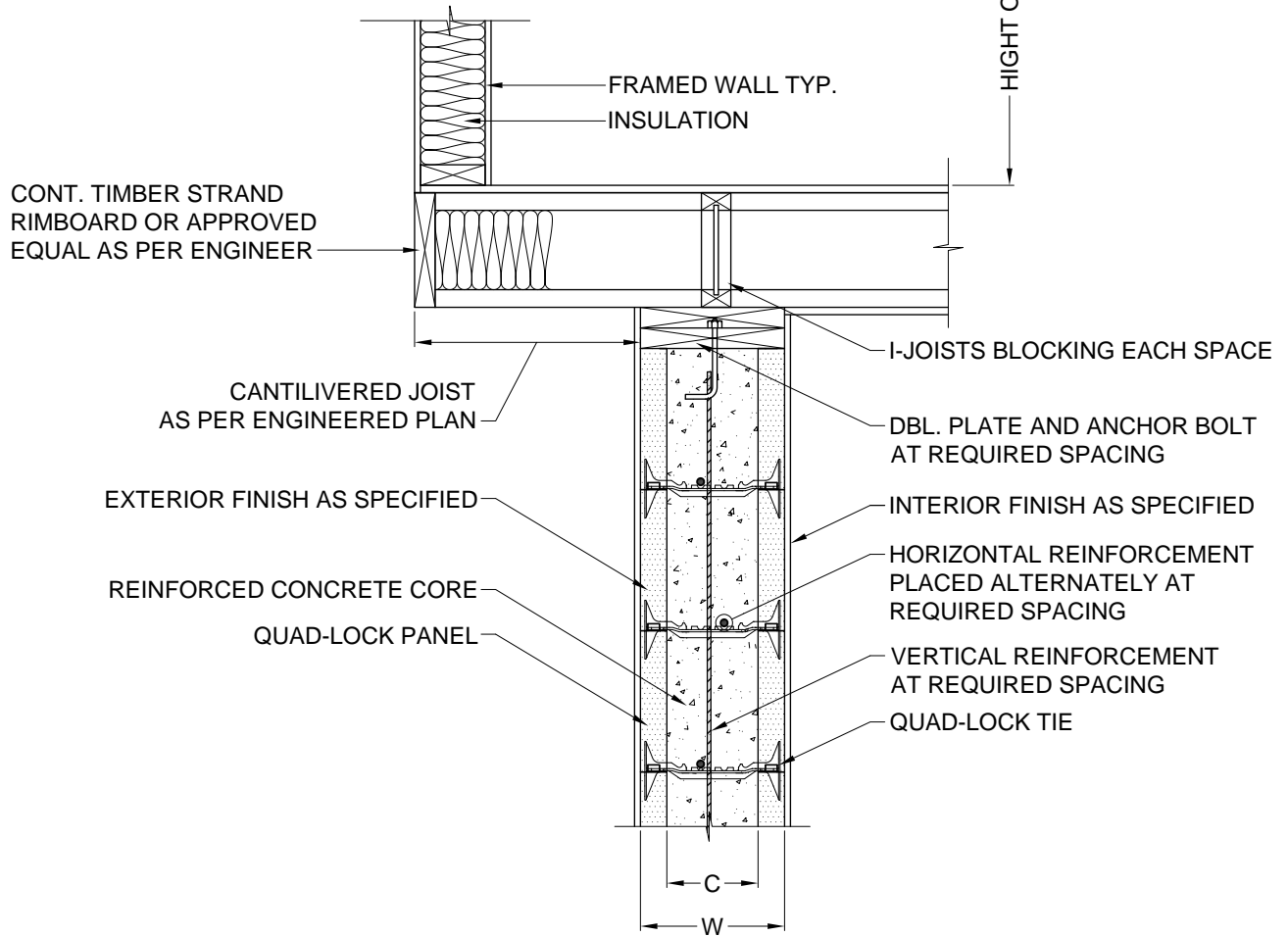
1 SECTION DETAIL 2.7 3/4" = 1'
