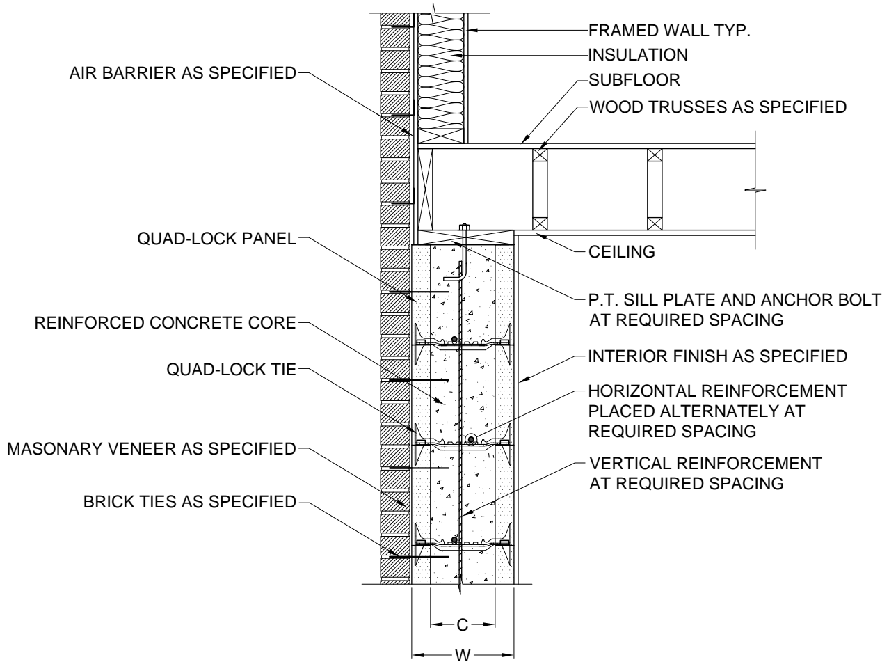
1 SECTION DETAIL 2.6 3/4" = 1'
