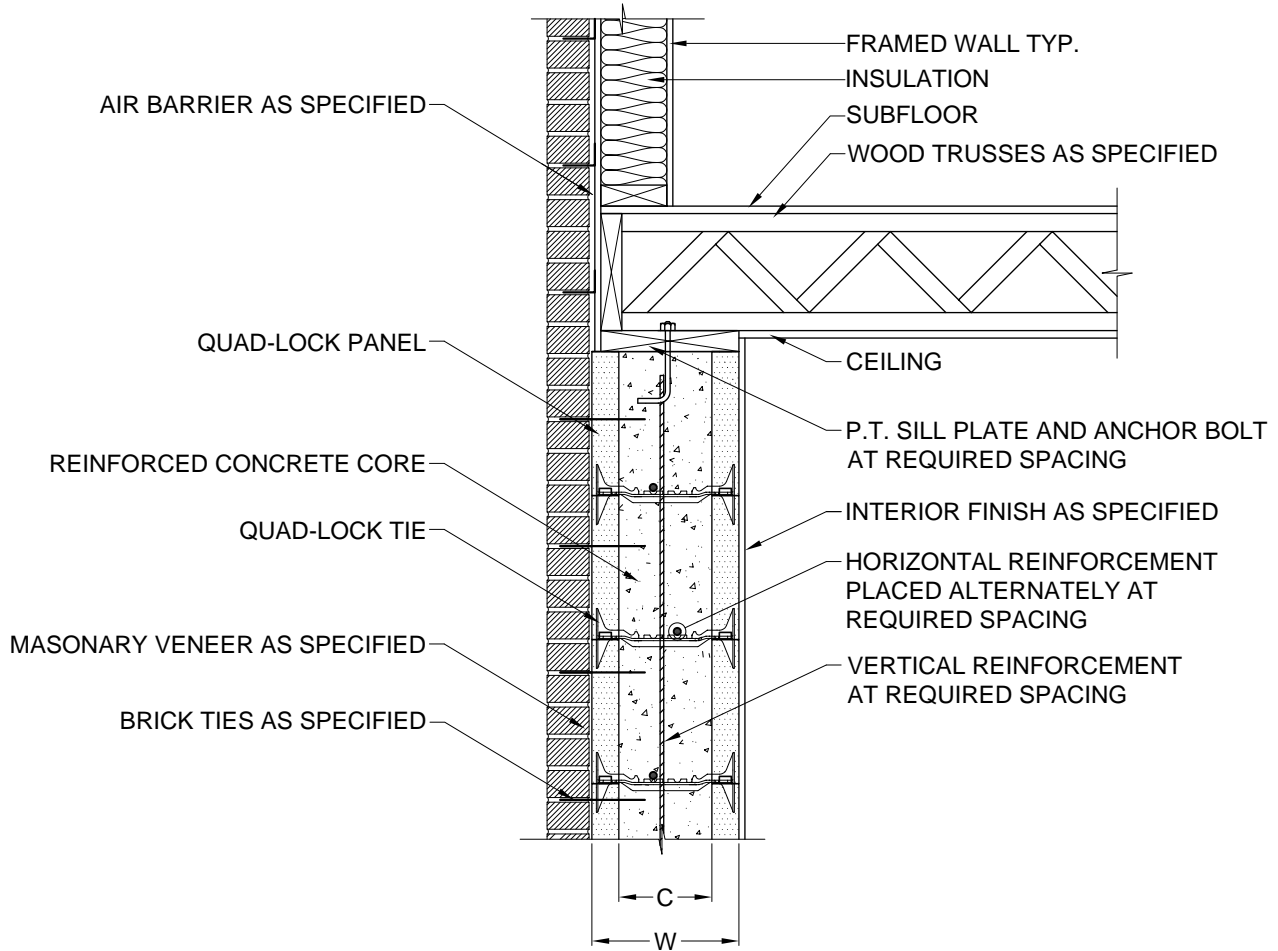
1 SECTION DETAIL 2.5 3/4" = 1'
