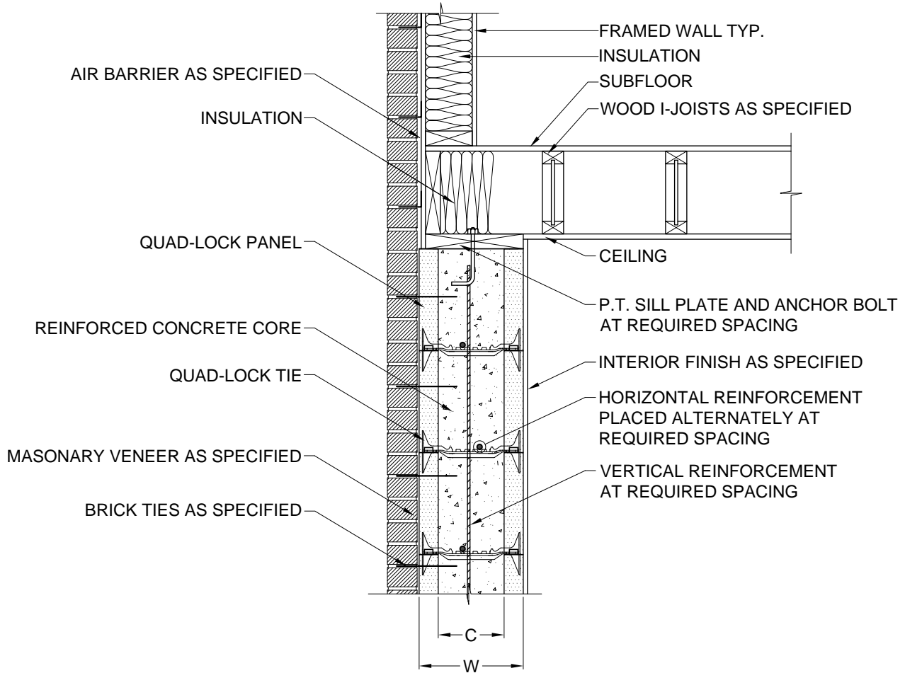
1 SECTION DETAIL 2.4 3/4" = 1'
