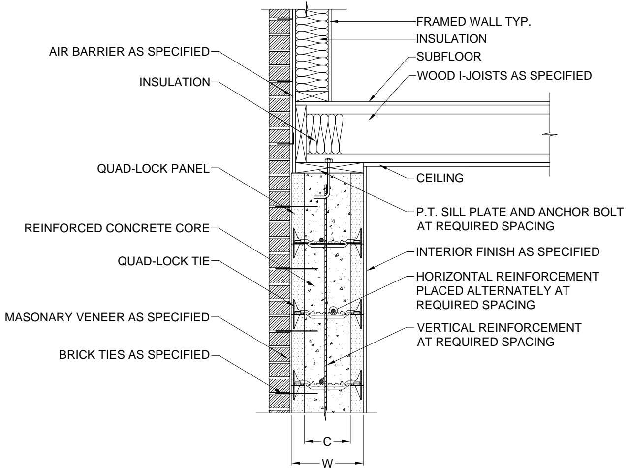
1 SECTION DETAIL 2.3 3/4" = 1'
