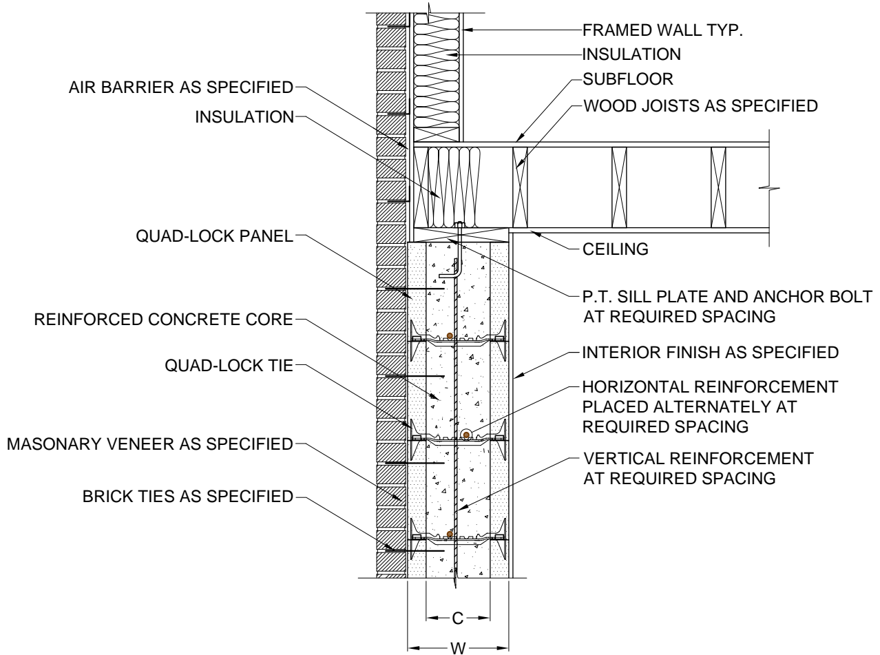
1 SECTION DETAIL 2.2 3/4" = 1'
