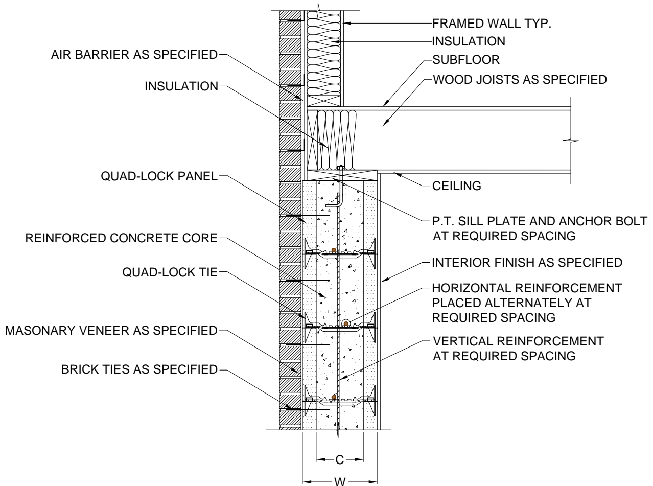
1 SECTION DETAIL 2.1 3/4" = 1'
