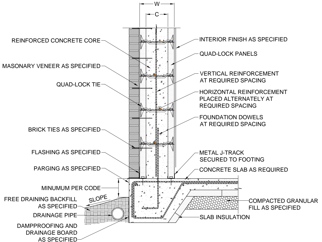
1 SECTION DETAIL 1.2 3/4" = 1'
