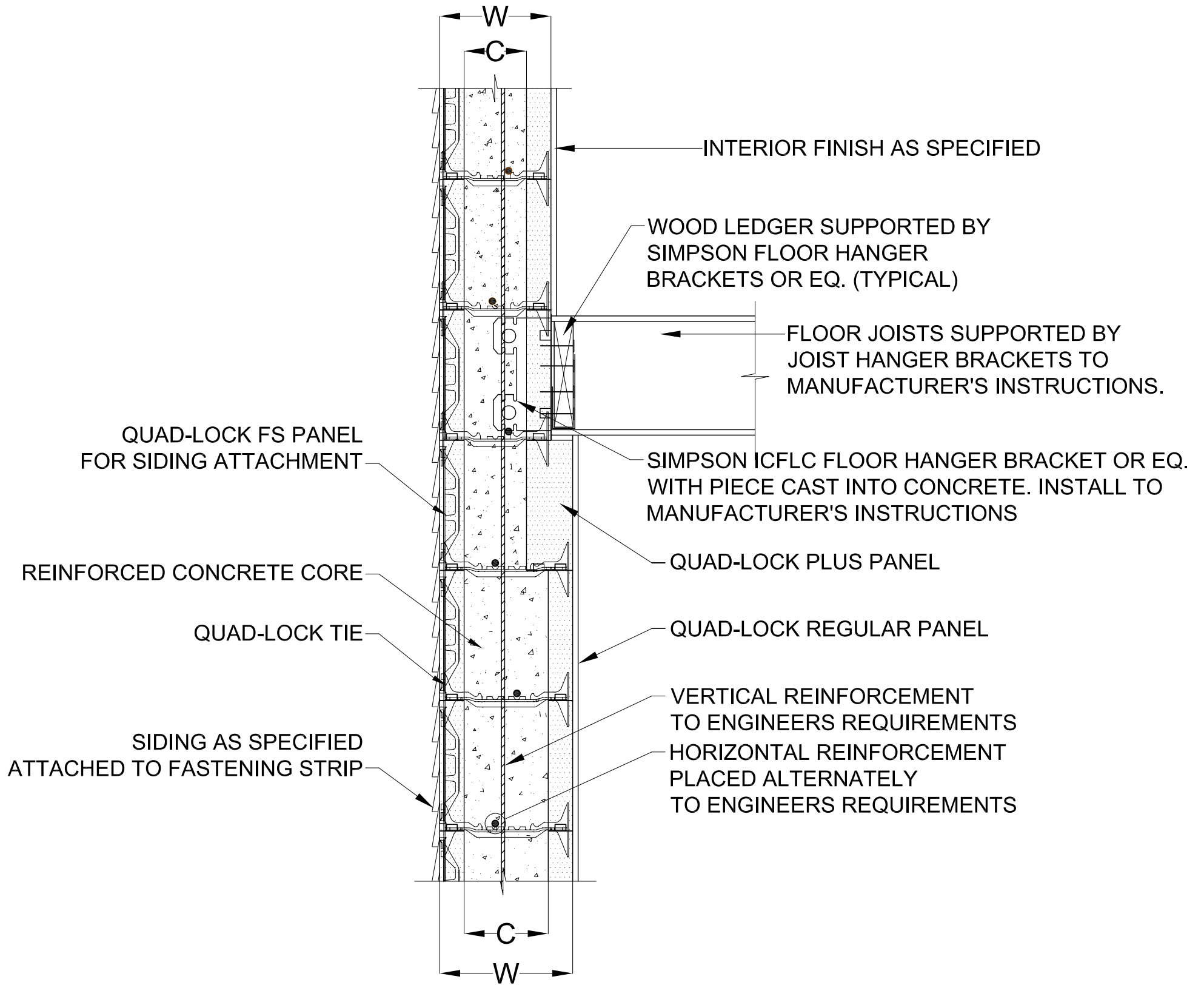
1 SECTION DETAIL 3.5
