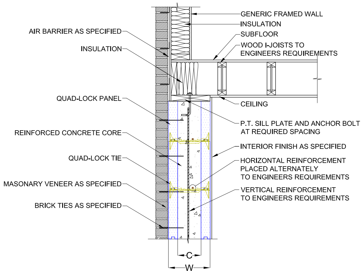
1 SECTION DETAIL 2.4
