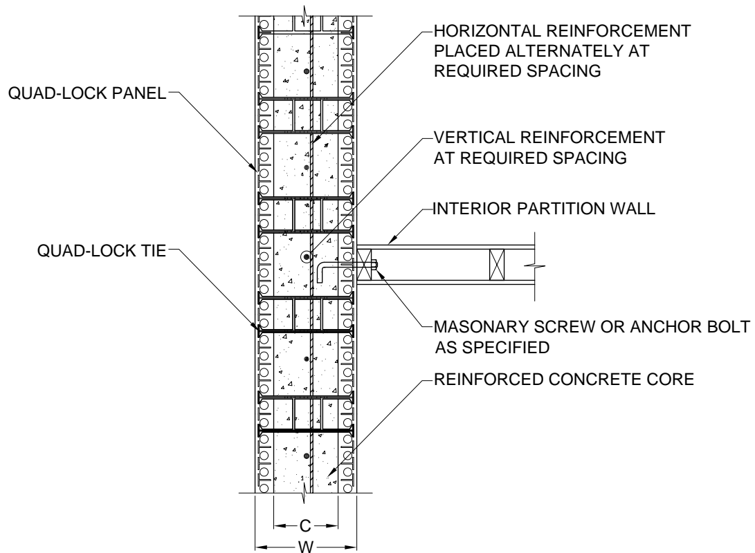
1 CONNECTION DETAIL 9.3 3/4" = 1'
