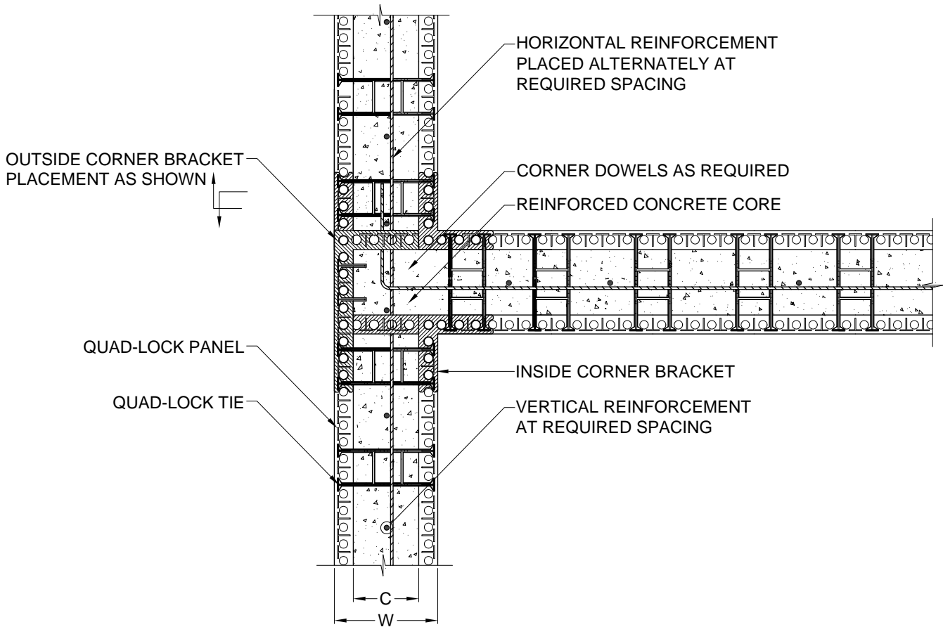
1 T-WALL DETAIL 8.3 3/4" = 1'
