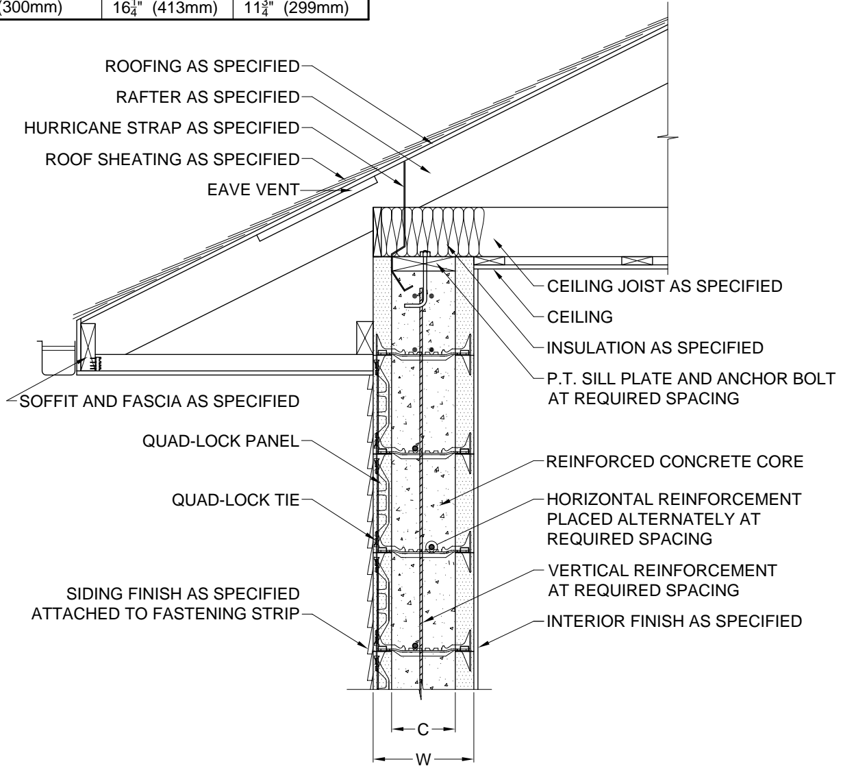
1 SECTION DETAIL 6.2 3/4" = 1'
