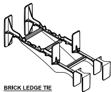
BRICK LEDGE TIE BLT
